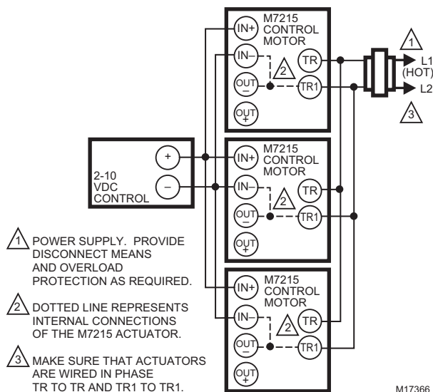
Fig. 4. Three M7215 Damper Motors connected in parallel.
