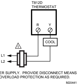
Fig. 8. T812D in cooling only application.
