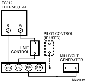
Fig. 5. Typical hookup to TS812A in millivolt system.
